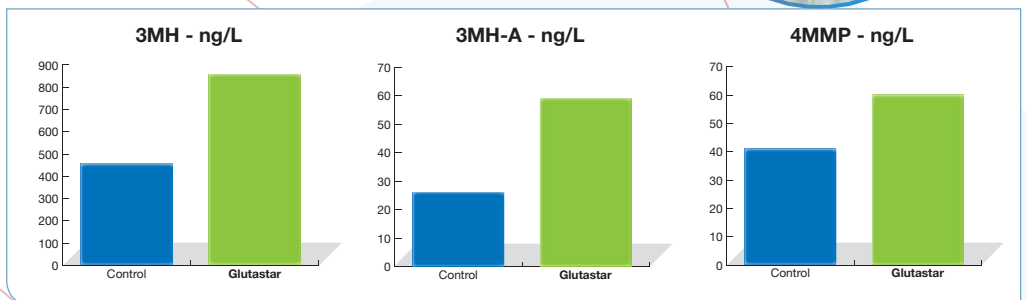
▲ Figure n°2: Comparative trial: Sauvignon blanc, Loire, 2018, analysis of volatile thiols at the end of AF
