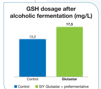
▲ Figure n°3: GSH dosages after AF, comparative trial, Sauvignon blanc 2018
